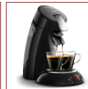
HD6556 ●
